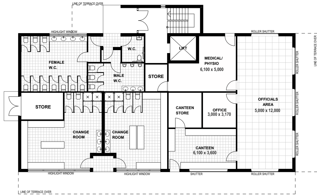
0. GROUND FLOOR 1:100
