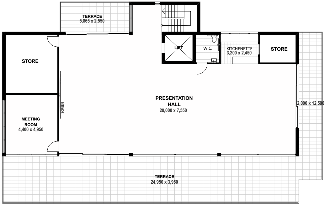
1. FIRST FLOOR 1:100
