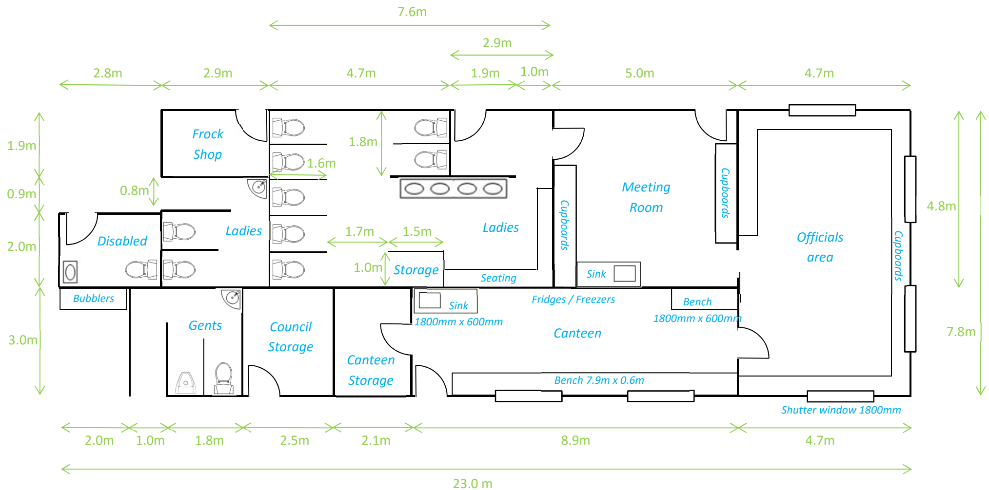
Canoon Rd Complex – floor plan
